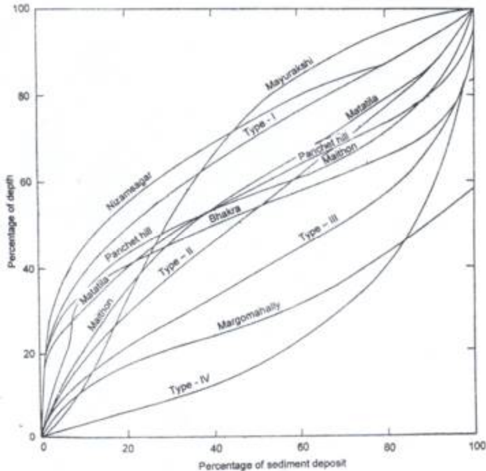
Fig.1 Showing Distribution of Sediments with Increasing Depths for Different Types of Reservoirs and the Distribution in some Major Reservoirs/Dams in India (Including Bhakra)
