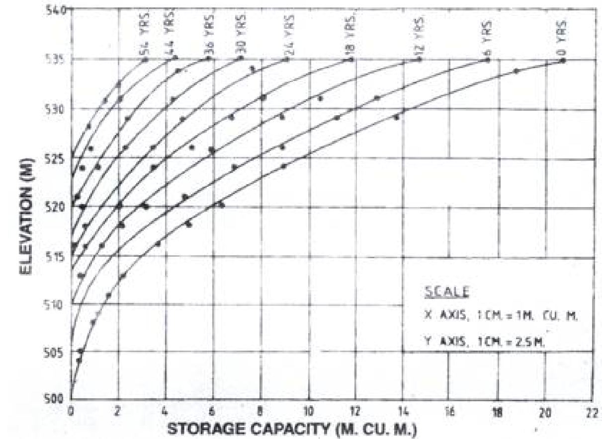
Fig.2 Showing Loss in storage Capacity in Kirichu Dam/Reservoir (in Sikim) at 6years interval
